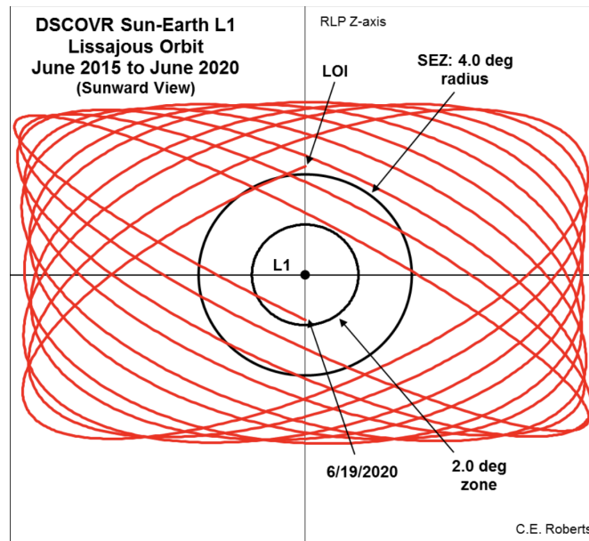
Figure 8: L_1 Lissajous orbit of sun-earth system
