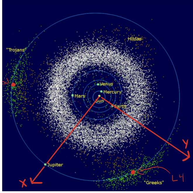
Figure 4: The green dots in the picture are the Trojan asteroids, they behave almost exactly as predicted in the CR3BP, and in Sun-Jupiter system, we have \mu = 0.00095 , and e = 0.0487 . The group of asteroid near L_4 are called Greek Camp and the group of asteroid near L_5 is called Trojan camp. Isn't it nice? Source: Wikipedia
