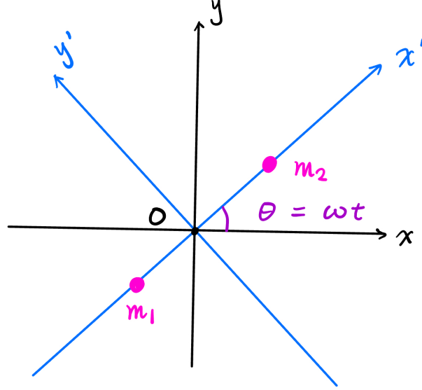
Figure 1: Rotating coordinate system x'y'
