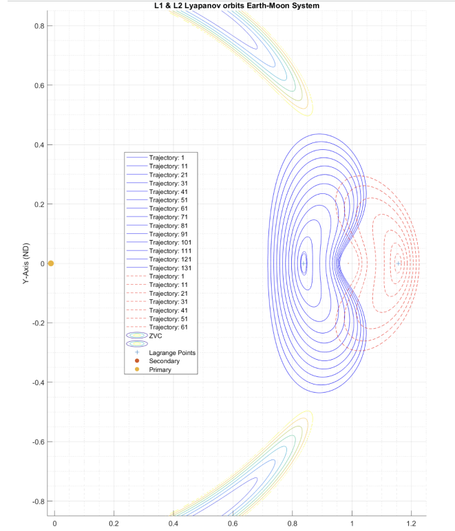
Figure 6: The Lyapunov orbits near L_1, L_2 of the earth-moon system
