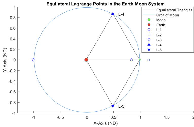
Figure 3: The other two Lagrange Points of the Earth-Moon system, denoted by L_4 and L_5 .
