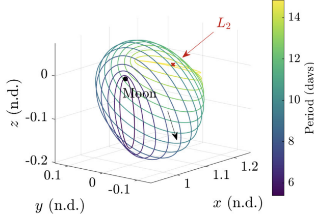
Figure 7: The Halo Orbits around L_2 of the earth-moon system. Source: Leveraging Intermediate Dynamical Models for Transitioning from the Circular Restricted Three-Body Problem to an Ephemeris Model
